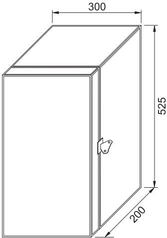
Amplifier with closed flight case
