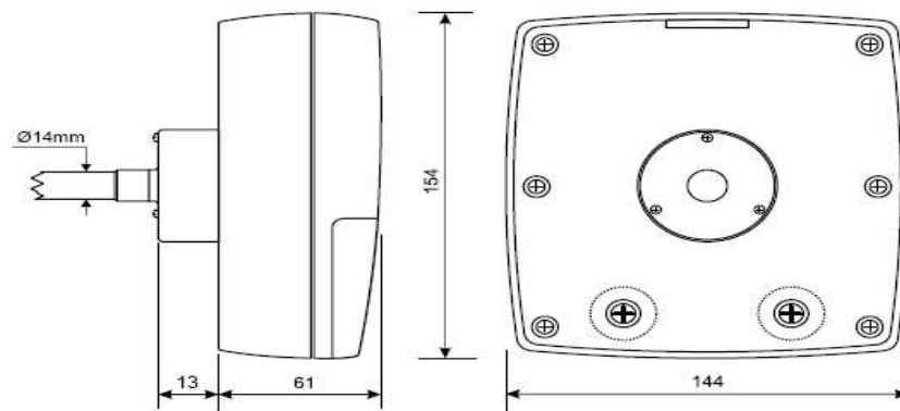
Version HD2717T0... for horizontal probes
