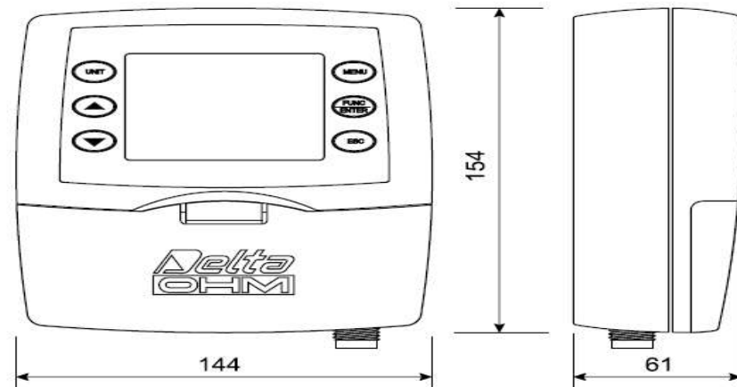
Versions HD2717Tx.xx for vertical probes or with cable
